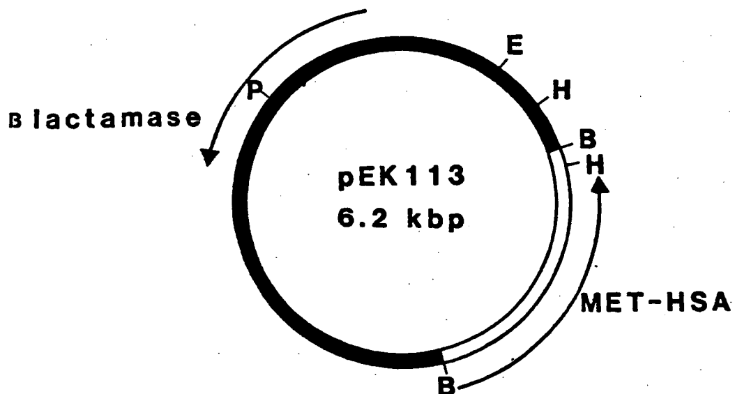
Fig 6 Plasmid pEK113
